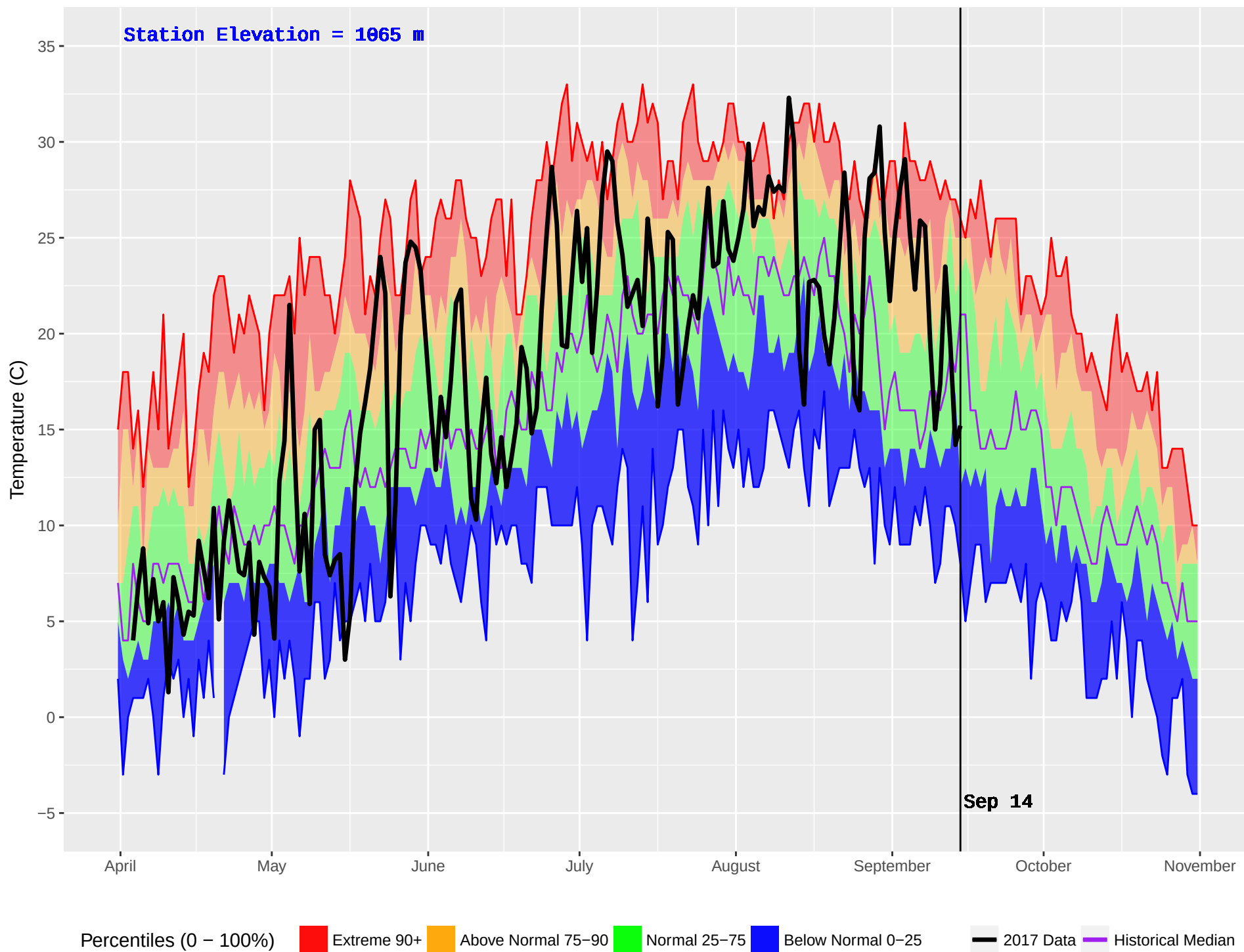
ASPEN GROVE (302) : Historical (1998–2016) and Current (2017) Noon Temperature
